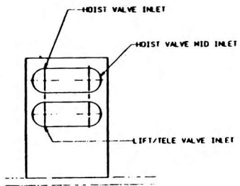
VIEW E-E
